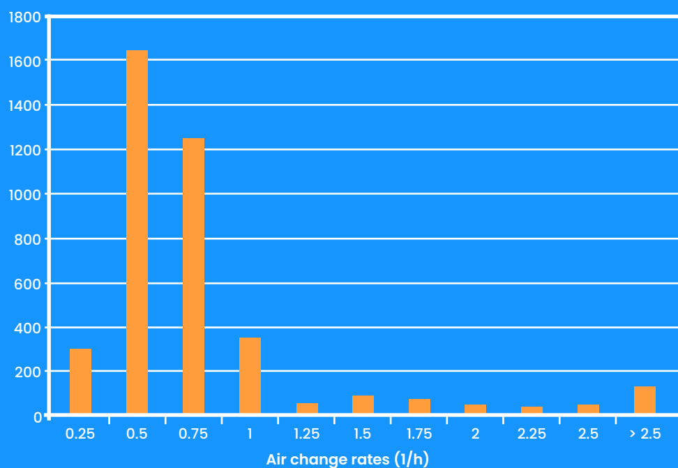
Fig. 4 Distribution of air change rates over one year in an occupied town house (Wallace et al. 2001)
